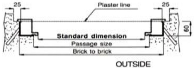
HORIZONTAL SECTION
