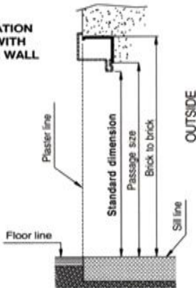
VERTICAL SECTION
