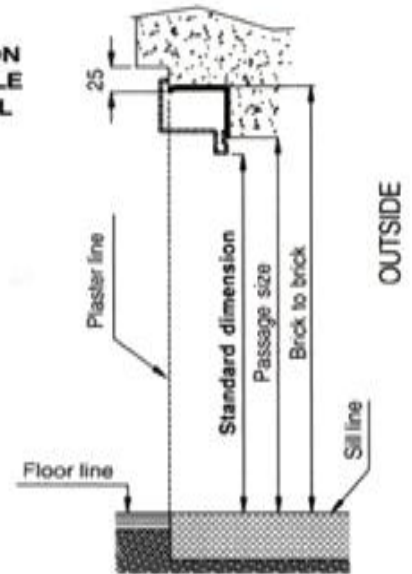
VERTICAL SECTION
